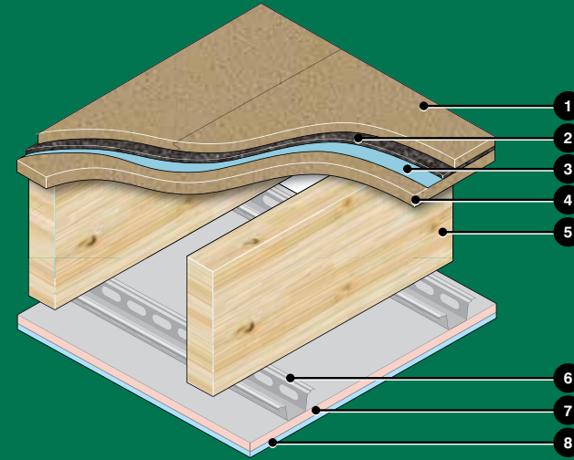
Ceiling Detail
