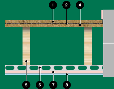
Ceiling Detail
